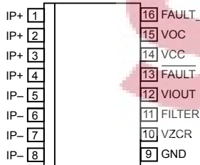
Pinout Diagram
